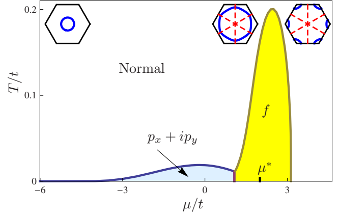
FIG. 2. (Color online) The phase diagram for spinless fermions on a triangular lattice with nearest-neighbor hoppings and attraction ( g/t=1 ). The bottom of the band is located at \mu=-6t and the top is at \mu=3t ; \mu^*=2t corresponds to a van Hove singularity. Two SC phases with (p_x+ip_y) - and f -wave symmetries are present. They are separated by a first-order phase transition at \mu_{\text{cr}}/t \approx 1.057 . The insets (left to right) are the FSs for \mu < \mu^* , \mu \leq \mu^* , and \mu > \mu^* and the dashed lines indicate the nodal directions of the f -wave SC.
